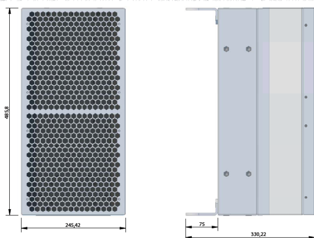
↑pic. DIMENSIONS M-215X
