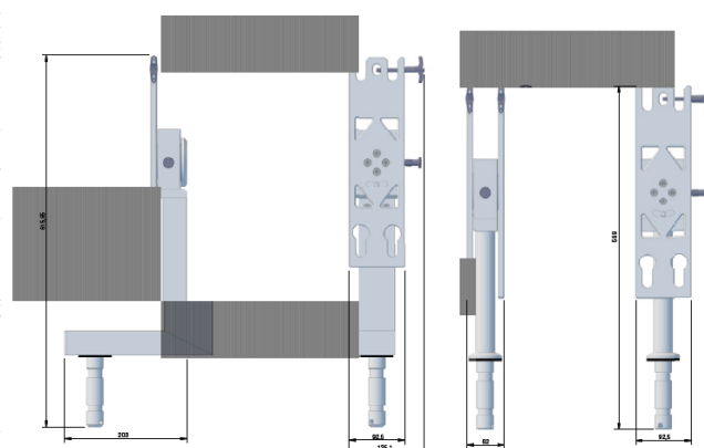
Quick mount for tripods and Monopole
